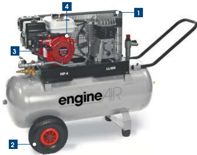
ENGINEAIR B2800B/100 4HP
