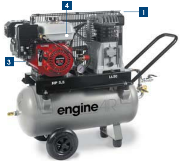
ENGINEAIR B3800B/50 5,5HP
