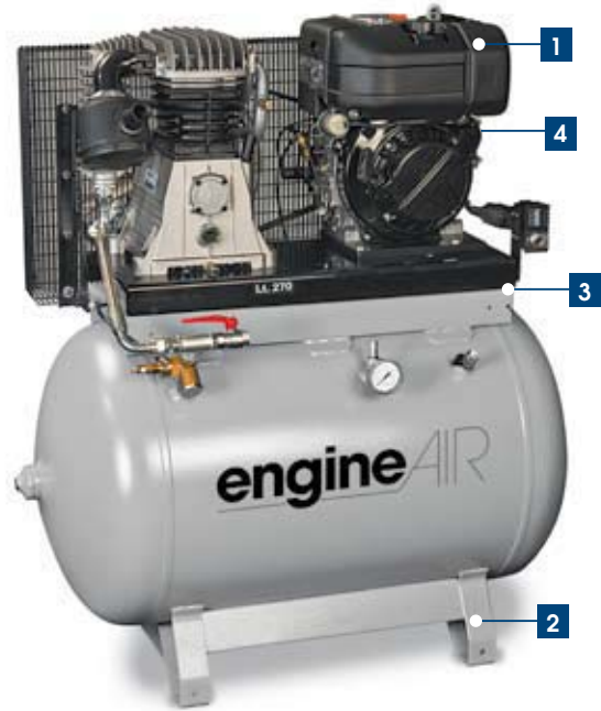
ENGINEAIR B6000/270 7HP DIESEL
